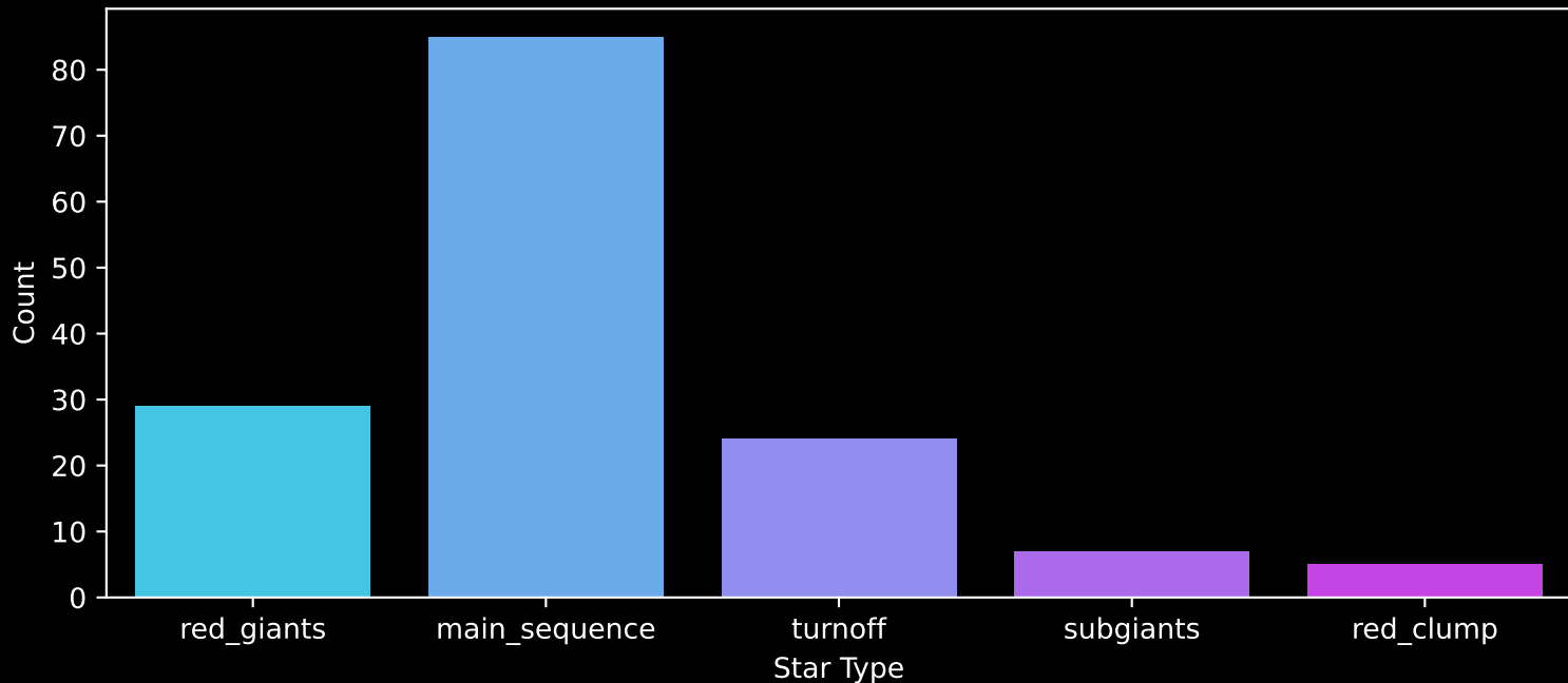
APOGEE DR17 Field: [043+44_MGA] Count plot of Star Type
