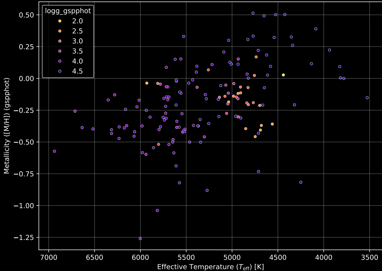
APOGEE DR17 Field: [043+44_MGA] Stellar Population Parameters (n= 150)
