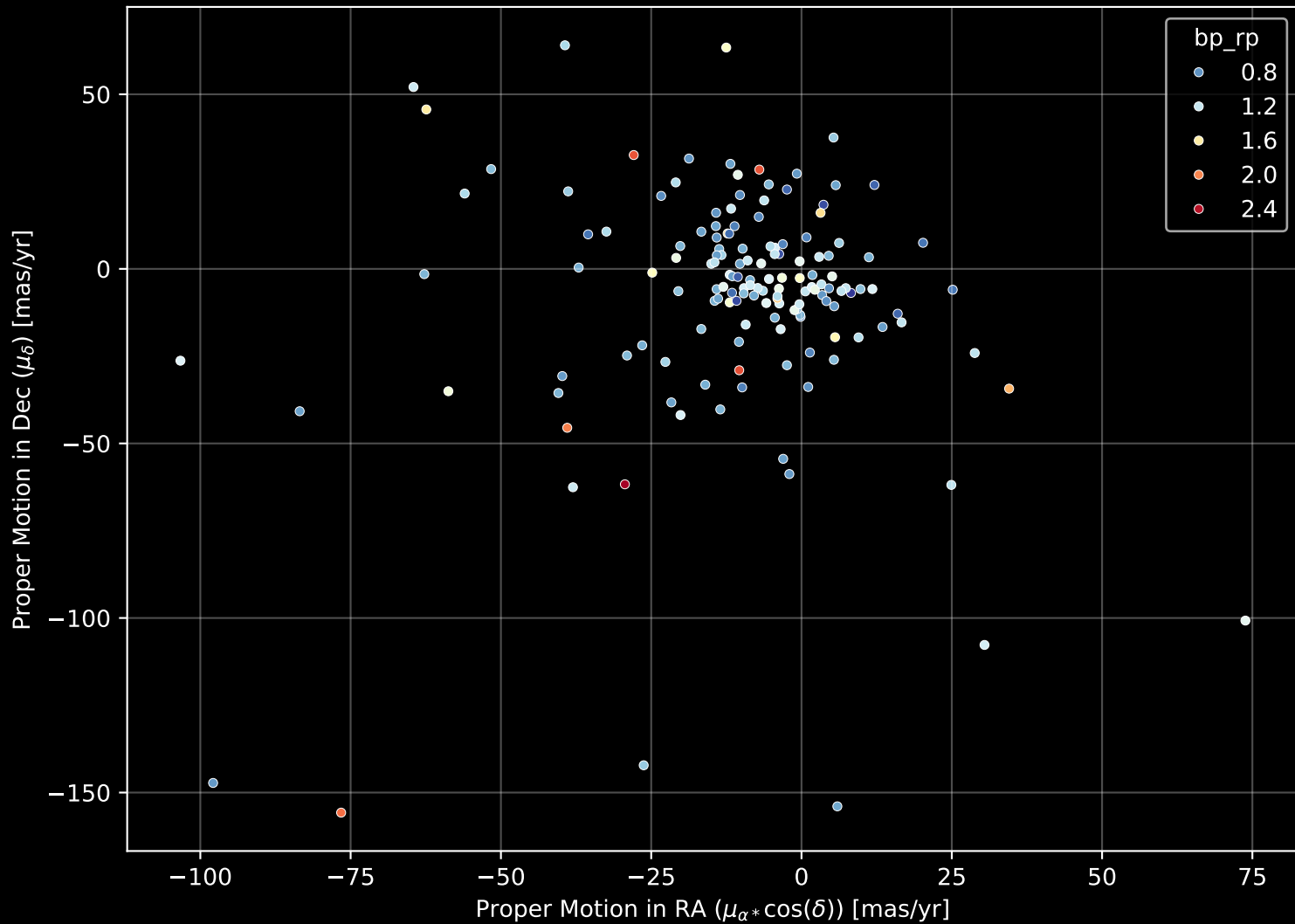
APOGEE DR17 Field: [043+44_MGA] Proper Motion Diagram (n= 150)
