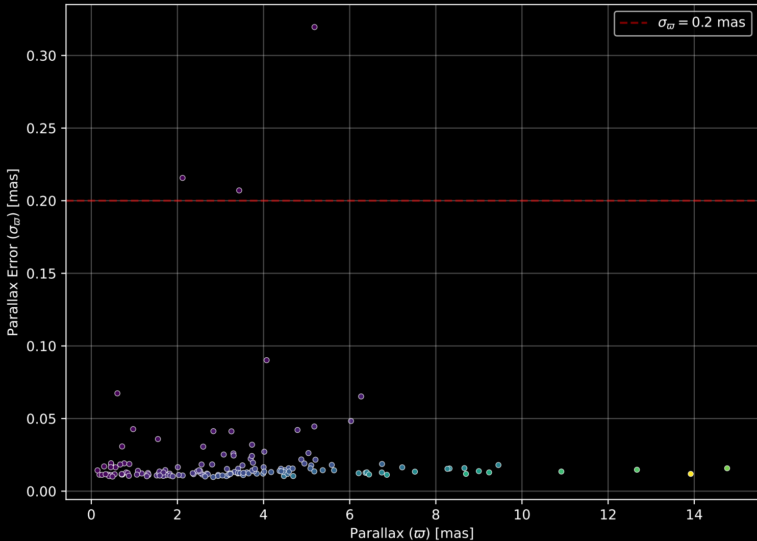
APOGEE DR17 Field: [043+44_MGA] Parallax Quality (n= 150)
