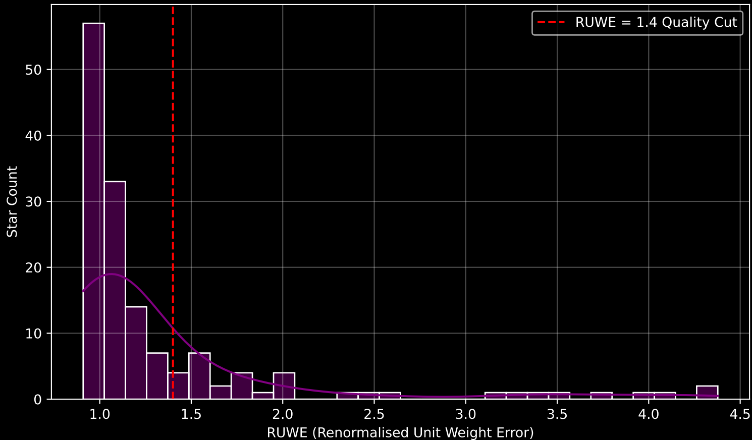
GAPOGEE DR17 Field [043+44_MGA] RUWE Distribution (n= 145)
