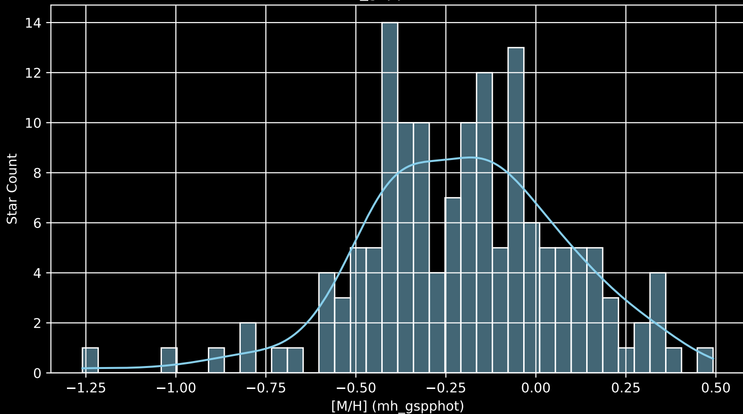
APOGEE DR17 Field: [043+44_MGA [M/H] (mh_gspphot) (n= 147)
